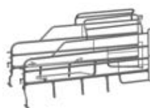
XL standard, with tiltable wings and upper structure, export L1 (incl.rear gate): 2400 mm } + 50 or L2 (incl.rear gate): 1975 mm } 100 mm
